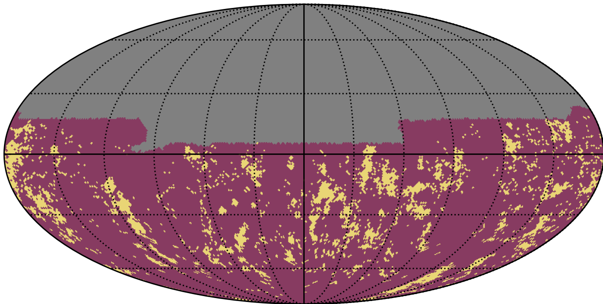
ddf_half_v3.4_10yrs u band: Gaps_3hr
