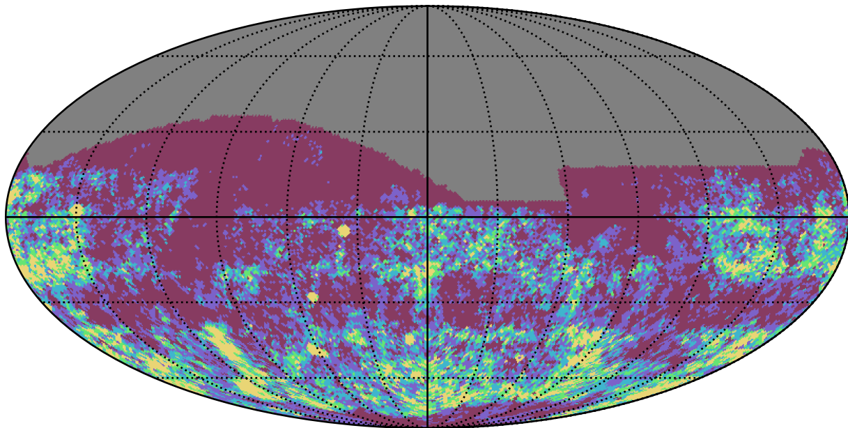
ddf_half_v3.4_10yrs i band: Gaps_3hr
