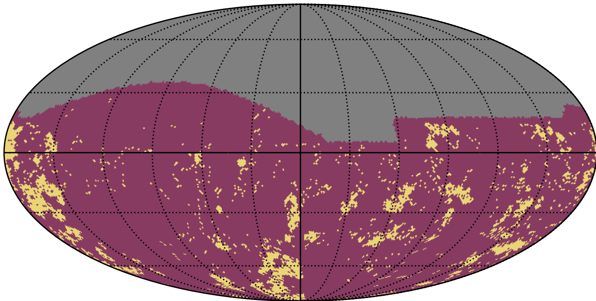
ddf_half_v3.4_10yrs g band: Gaps_3hr
