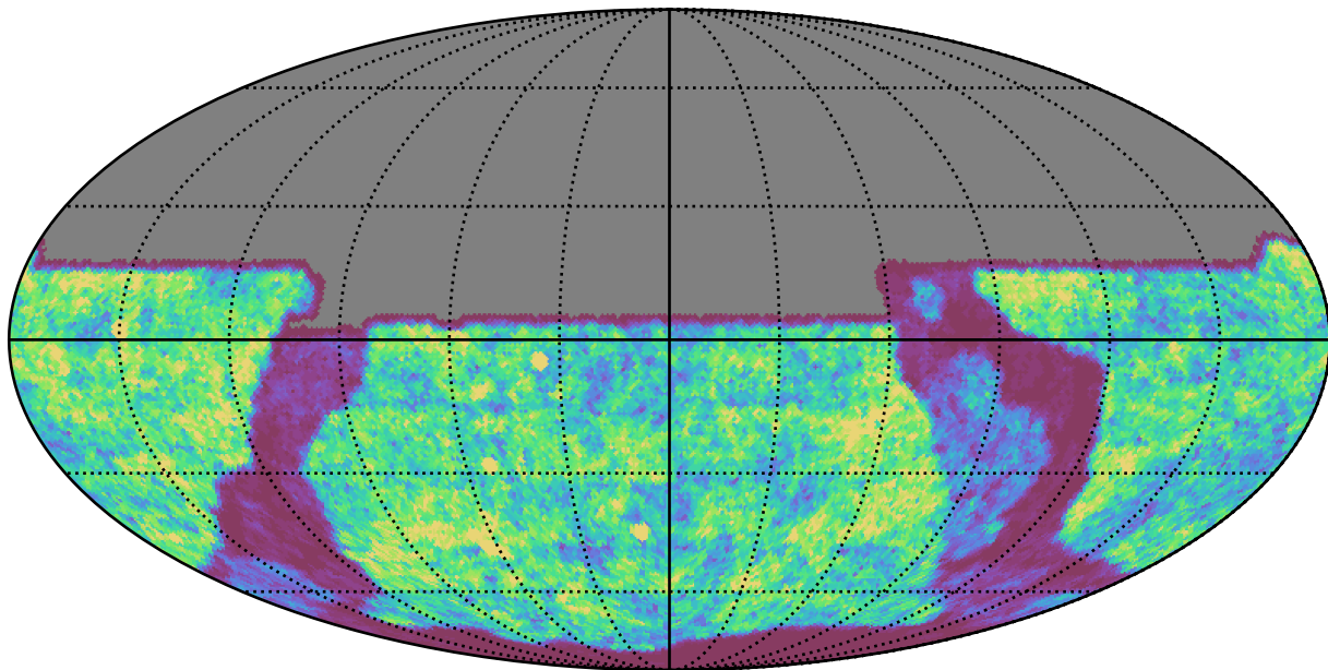
ddf_half_v3.4_10yrs y band: Gaps_24hr
