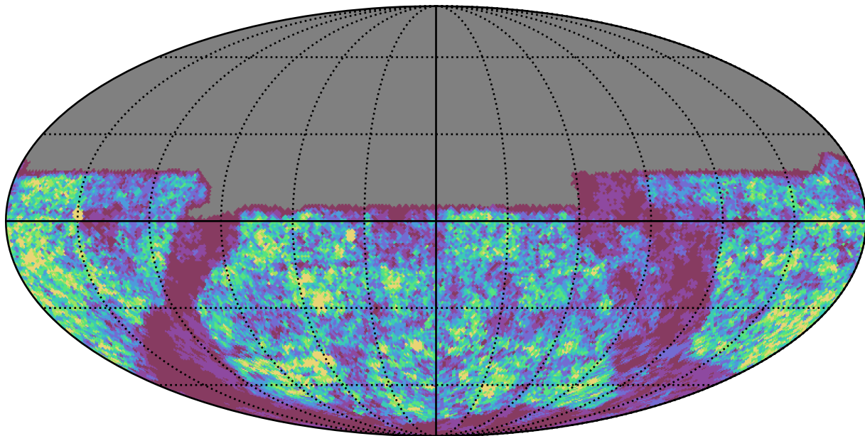
ddf_half_v3.4_10yrs u band: Gaps_24hr
