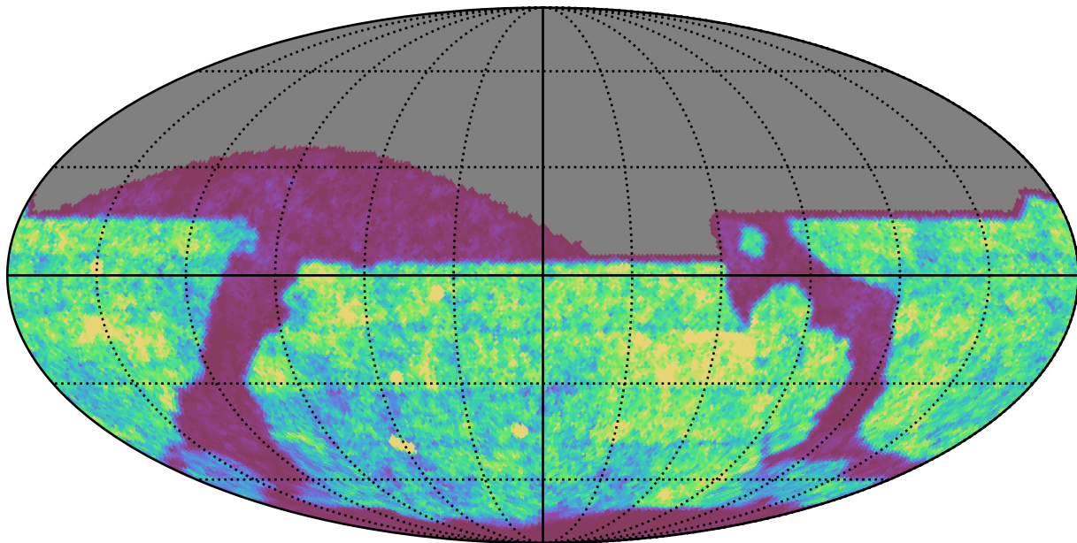
ddf_half_v3.4_10yrs r band: Gaps_24hr
