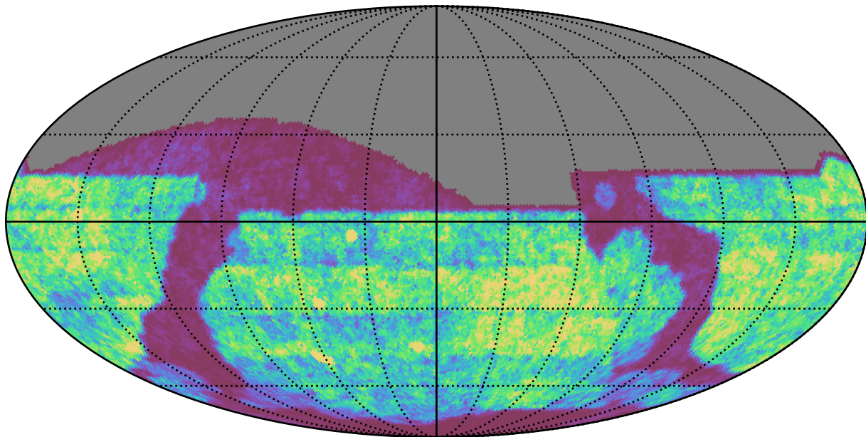
ddf_half_v3.4_10yrs i band: Gaps_24hr
