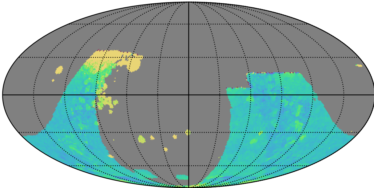
ddf_half_v3.4_10yrs : GalplaneTimePerFilter_combined_map_z
