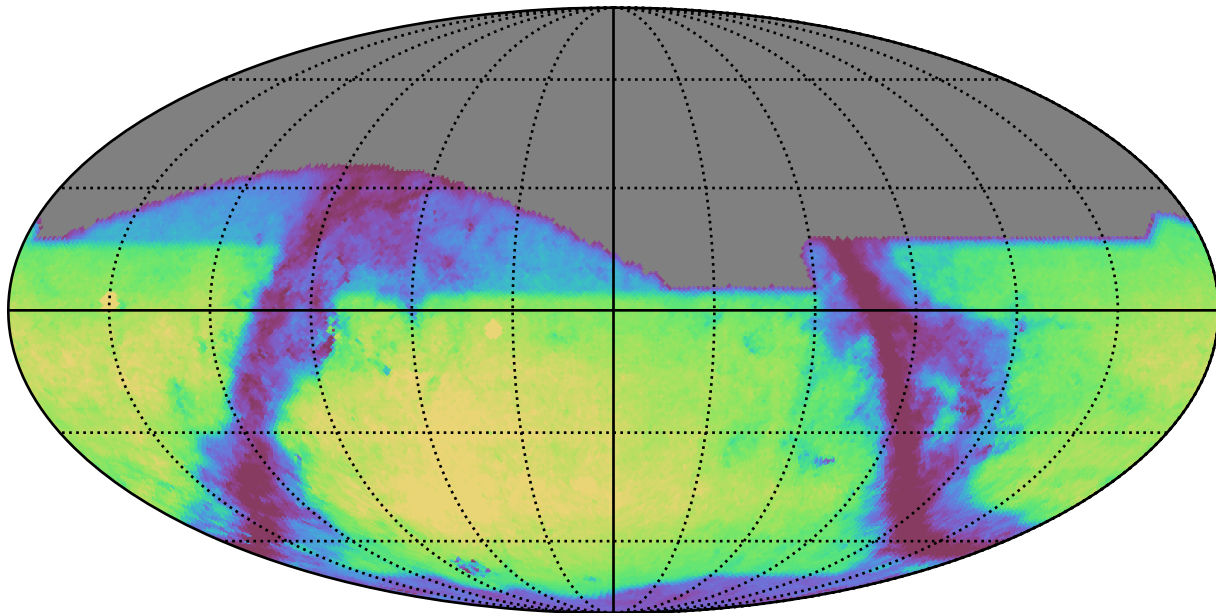
ddf_half_v3.4_10yrs r: GalaxyCountsMetricExtended
