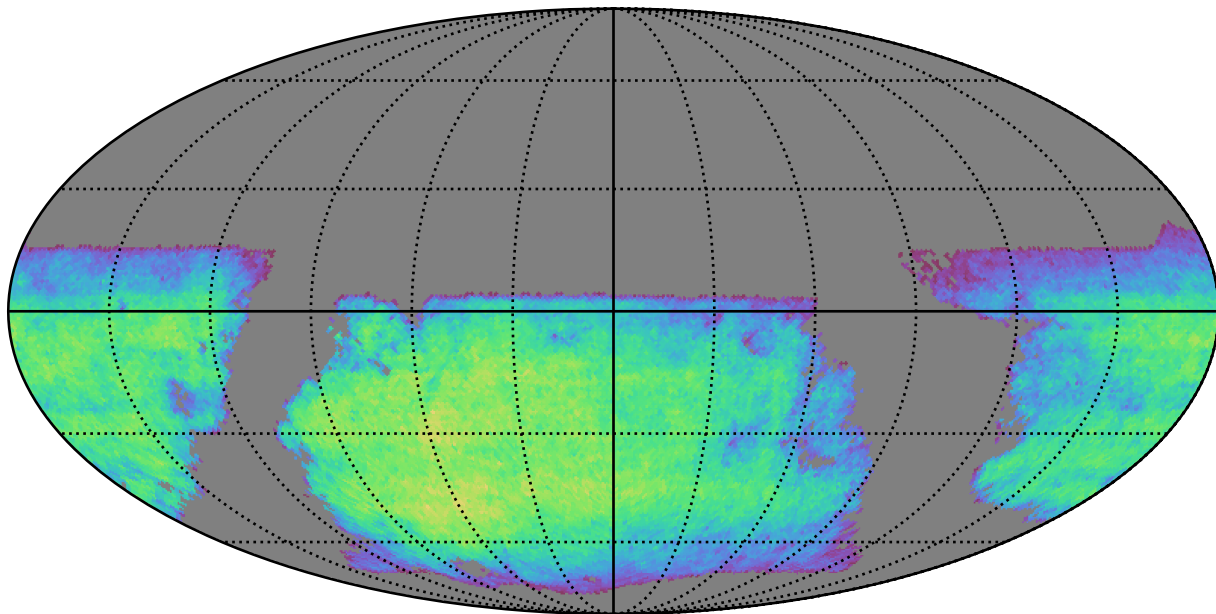
ddf_half_v3.4_10yrs i band non-DD year 8: ExgalM5WithCuts
