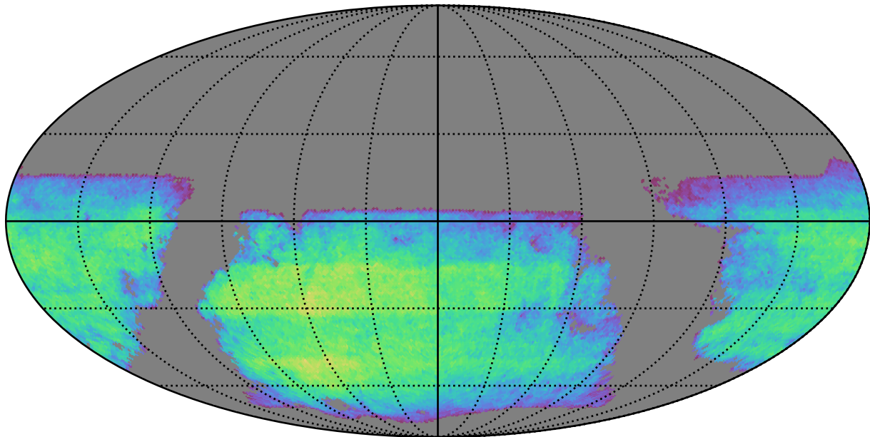
ddf_half_v3.4_10yrs i band non-DD year 7: Exgal5WithCuts
