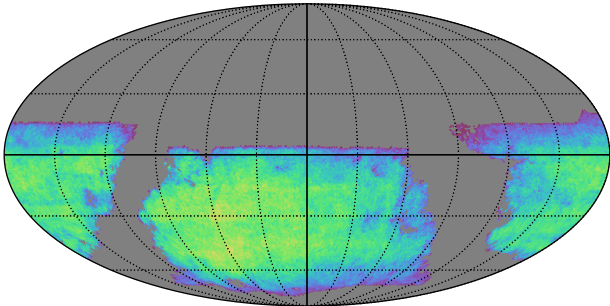
ddf_half_v3.4_10yrs i band non-DD year 6: ExgalM5WithCuts
