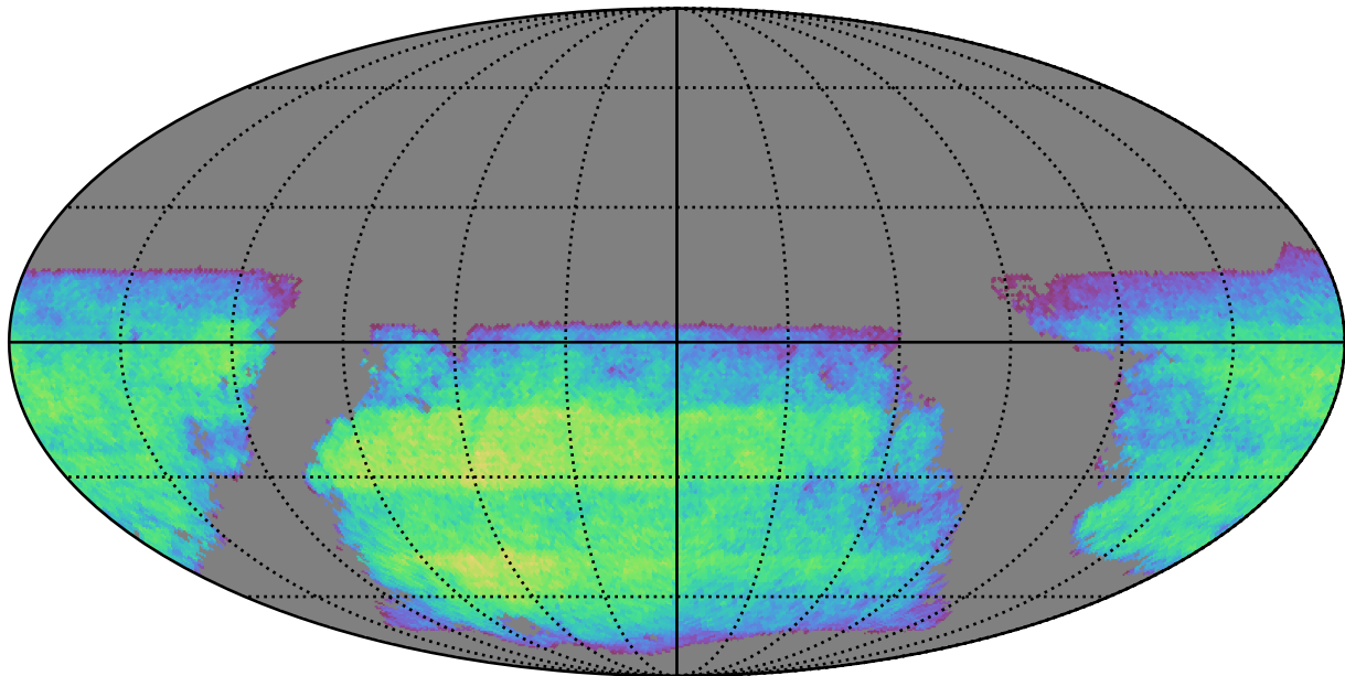
ddf_half_v3.4_10yrs i band non-DD year 5: ExgalM5WithCuts
