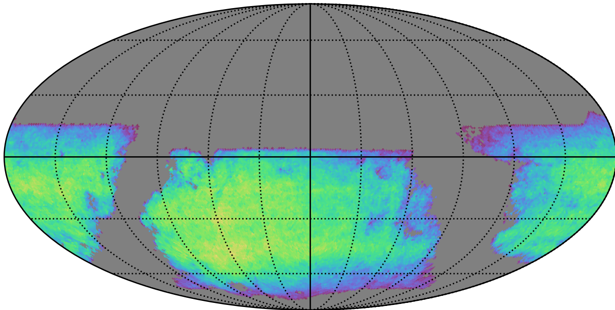
ddf_half_v3.4_10yrs i band non-DD year 10: ExgalM5WithCuts
