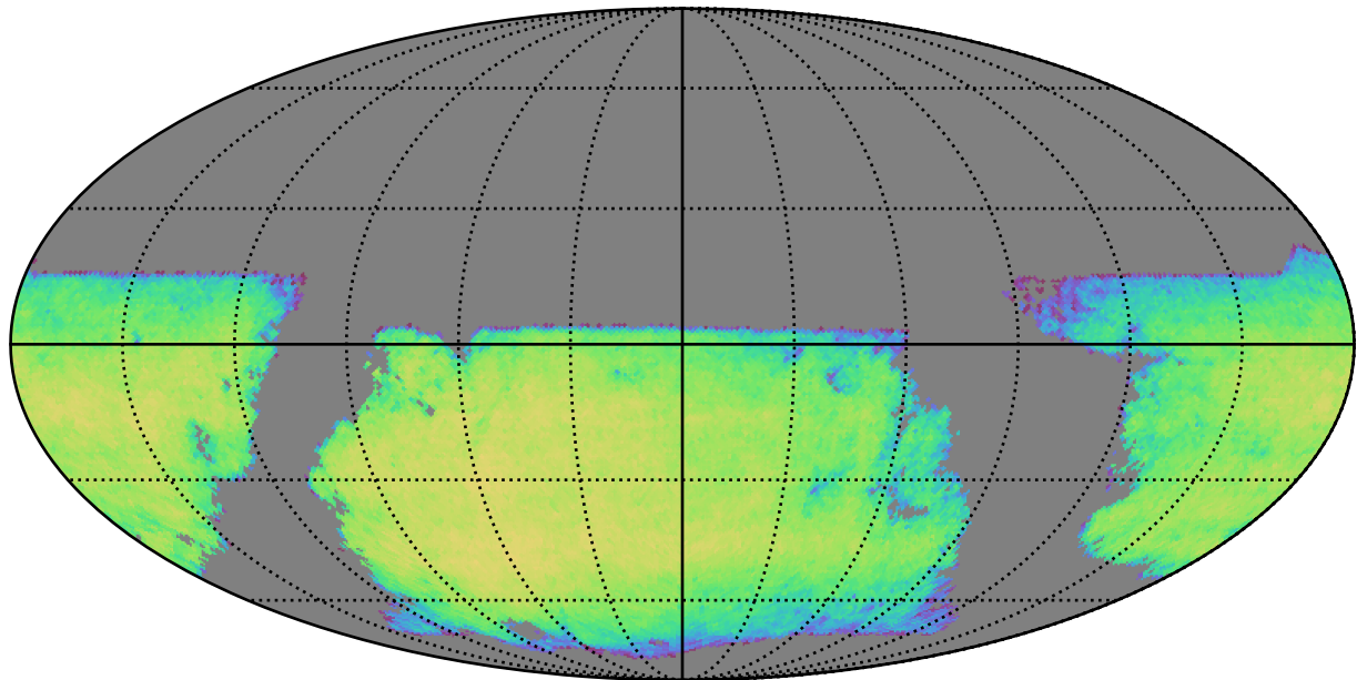
ddf_half_v3.4_10yrs i band galaxies non-DD: DepthLimitedNumGalaxiesMetric
