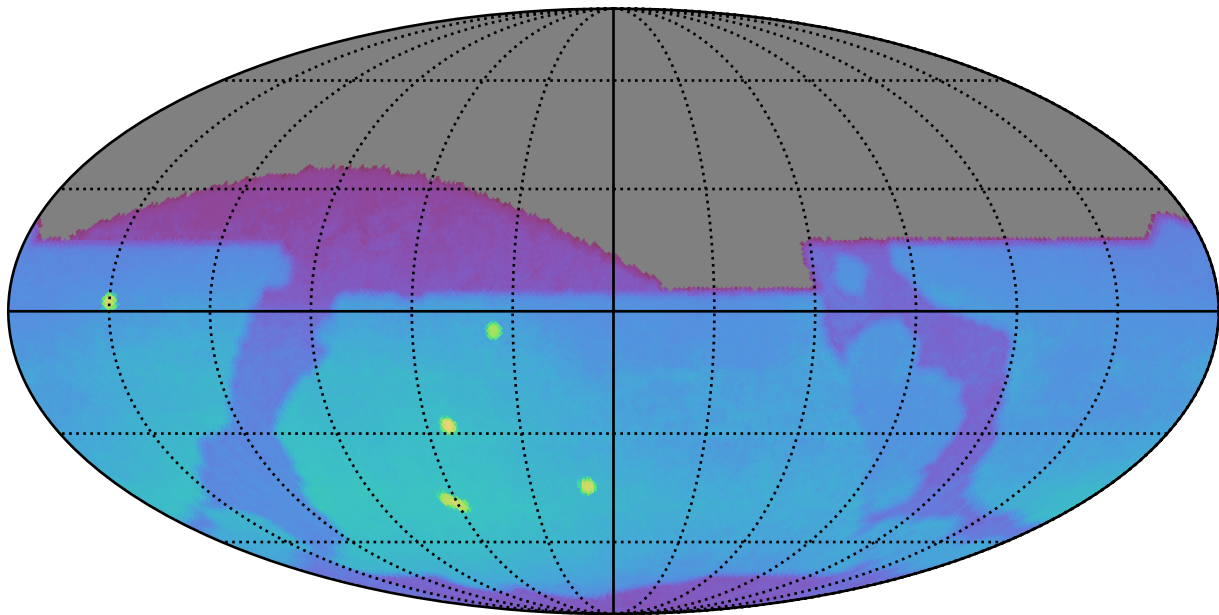
ddf_half_v3.4_10yrs : Brown Dwarf, L7
