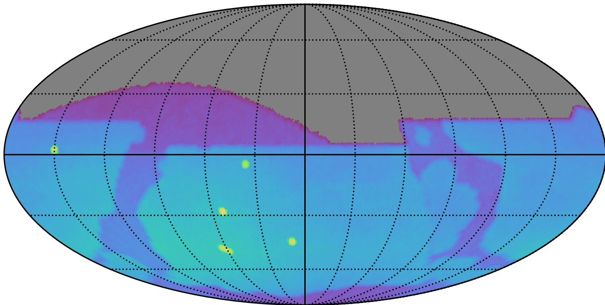
ddf_half_v3.4_10yrs : Brown Dwarf, L4
