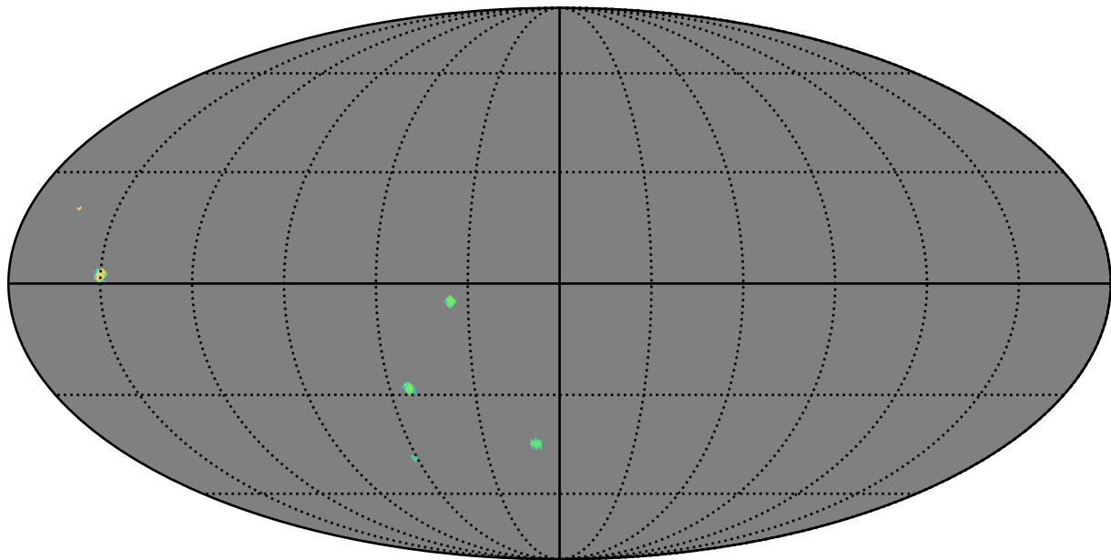
ddf_half_v3.4_10yrs z band: AGN_TimeLag_5_days
