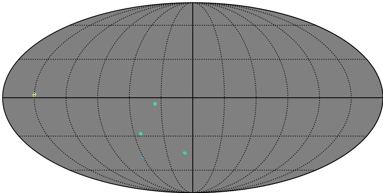
ddf_half_v3.4_10yrs r band: AGN_TimeLag_5_days
