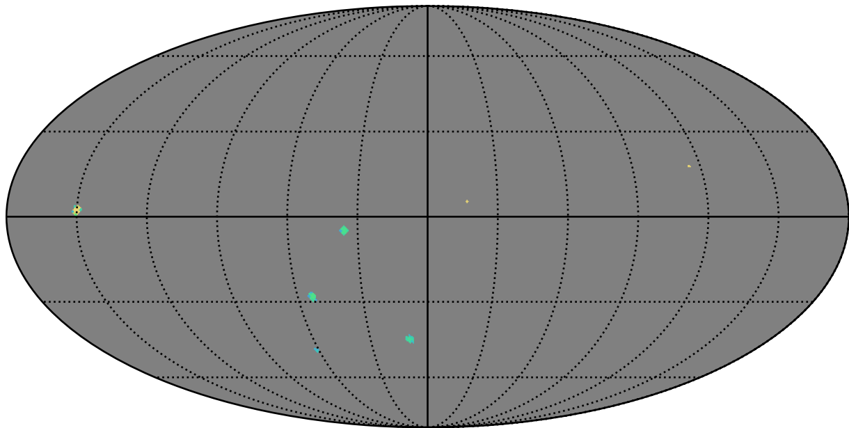
ddf_half_v3.4_10yrs i band: AGN_TimeLag_5_days
