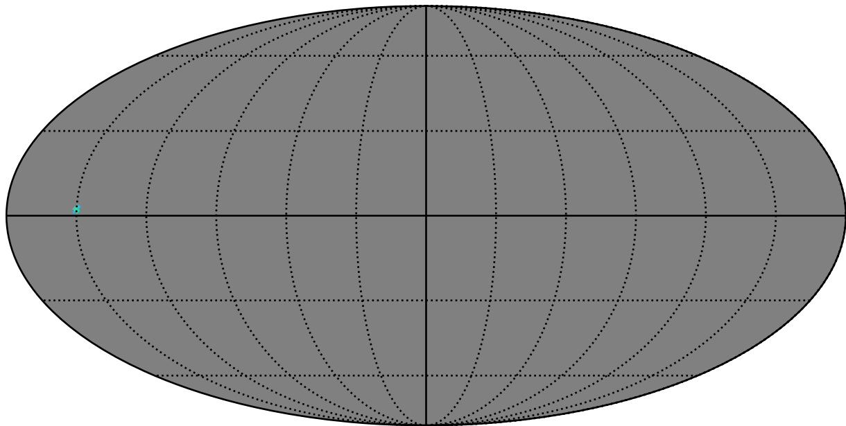
ddf_half_v3.4_10yrs g band: AGN_TimeLag_5_days
