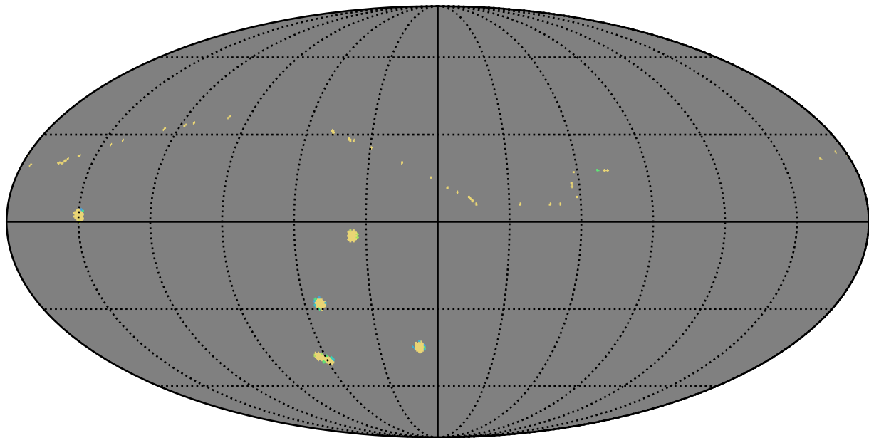
ddf_half_v3.4_10yrs all bands: AGN_TimeLag_5_days
