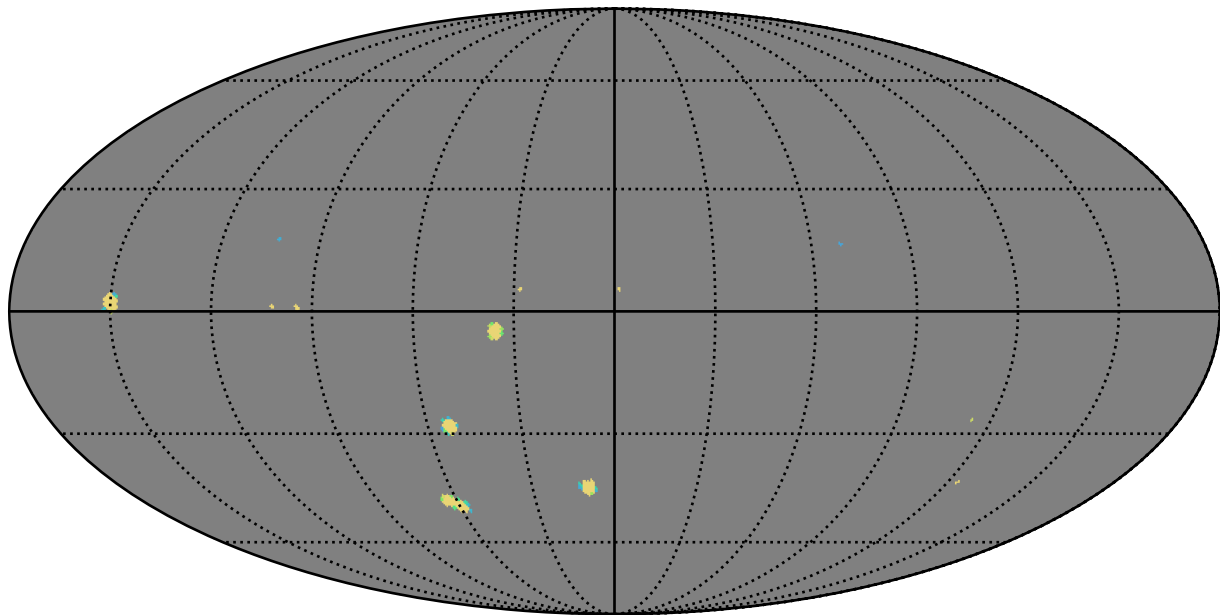
ddf_half_v3.4_10yrs u band: AGN_TimeLag_100_days
