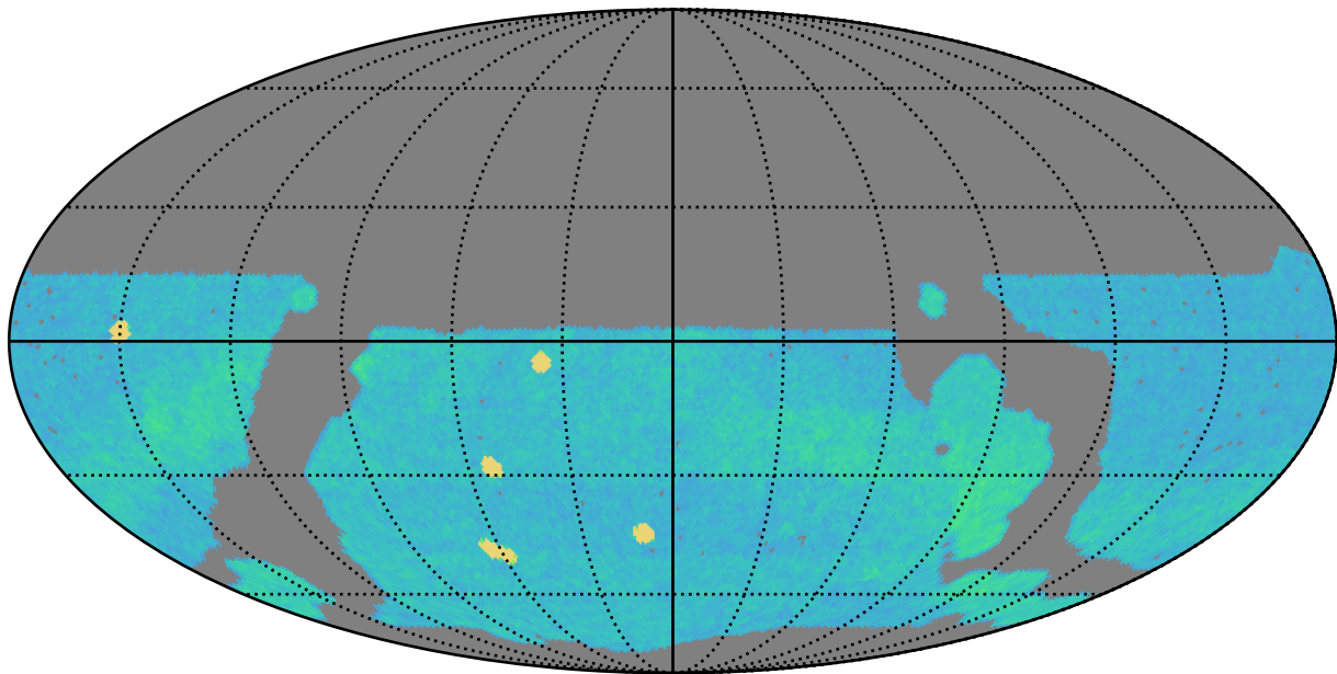
ddf_half_v3.4_10yrs r band: AGN_TimeLag_100_days
