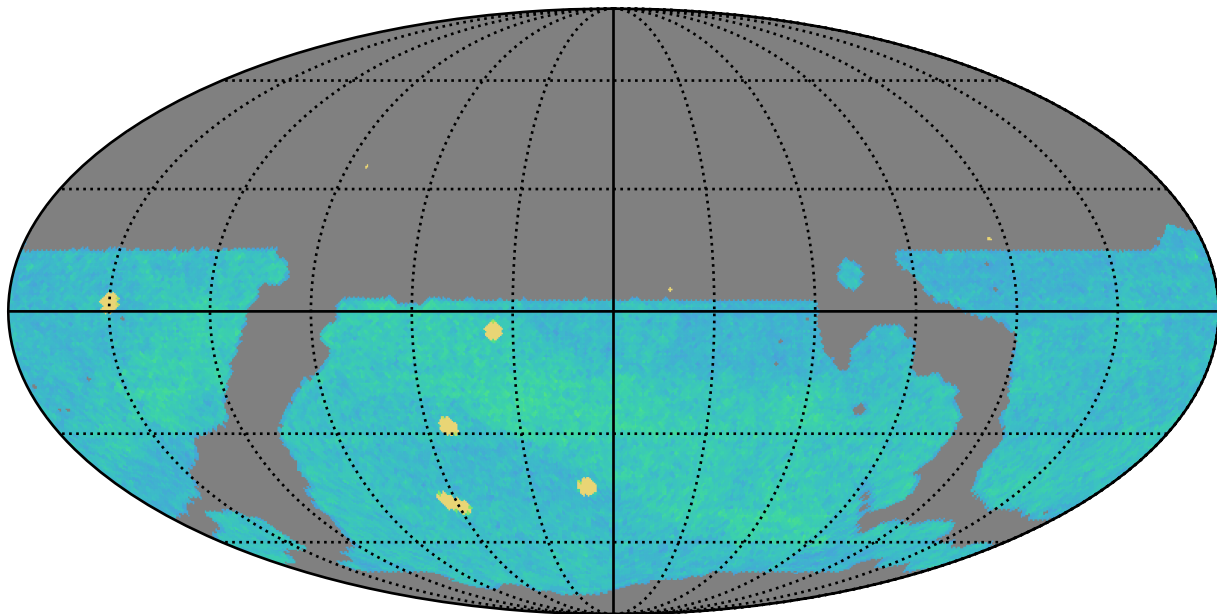
ddf_half_v3.4_10yrs i band: AGN_TimeLag_100_days
