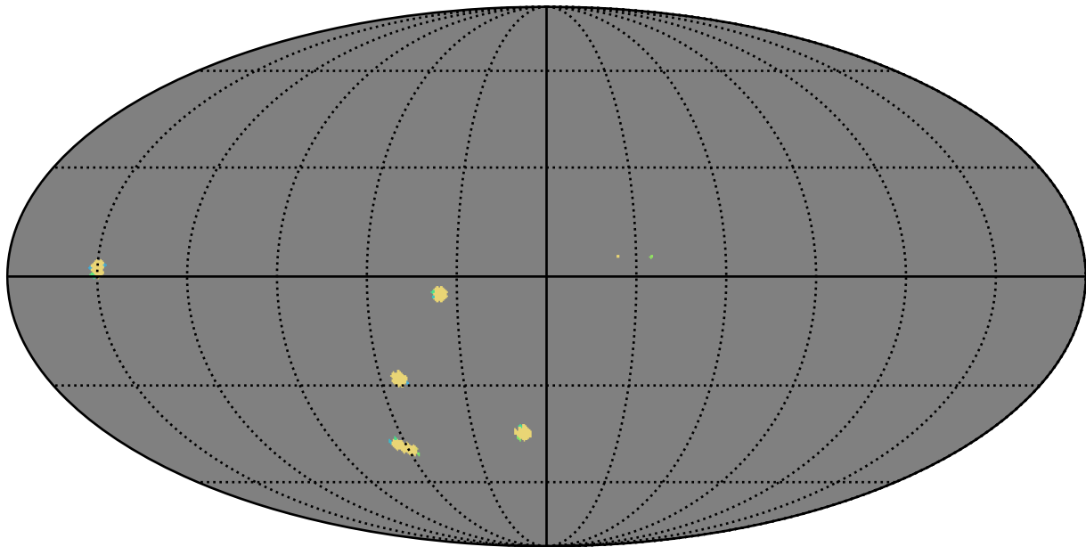
ddf_half_v3.4_10yrs g band: AGN_TimeLag_100_days
