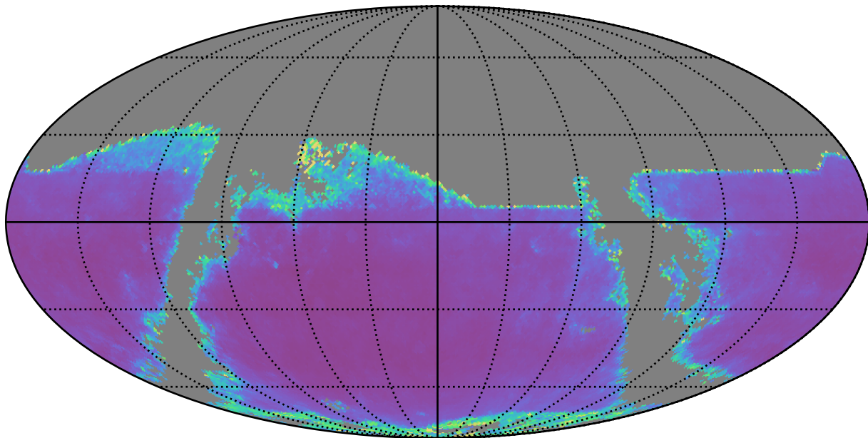
ddf_half_v3.4_10yrs r band: AGN SF_uncert
