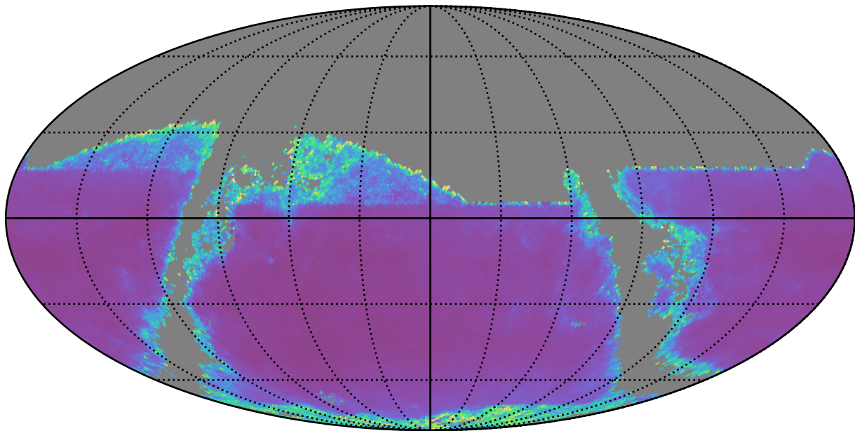
ddf_half_v3.4_10yrs i band: AGN SF_uncert
