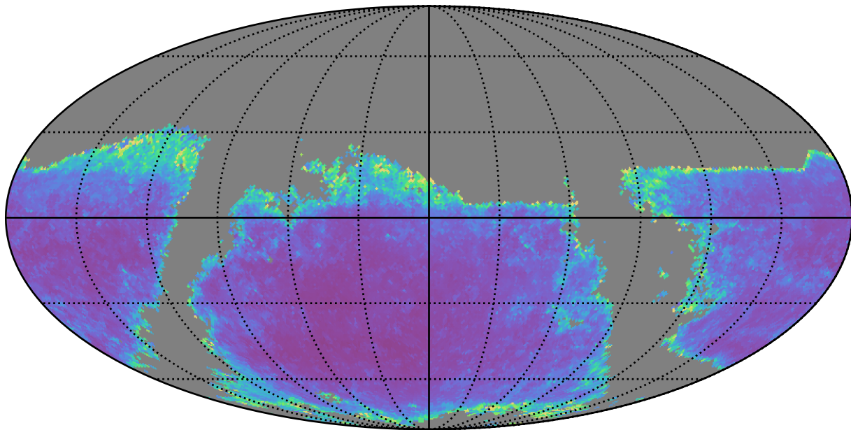
ddf_half_v3.4_10yrs g band: AGN SF_uncert
