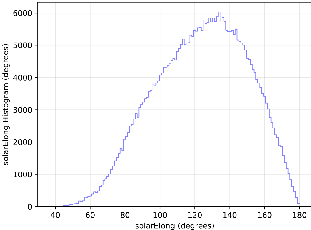
ddf_half_v3.4_10yrs WFD y band: solarElong Histogram
