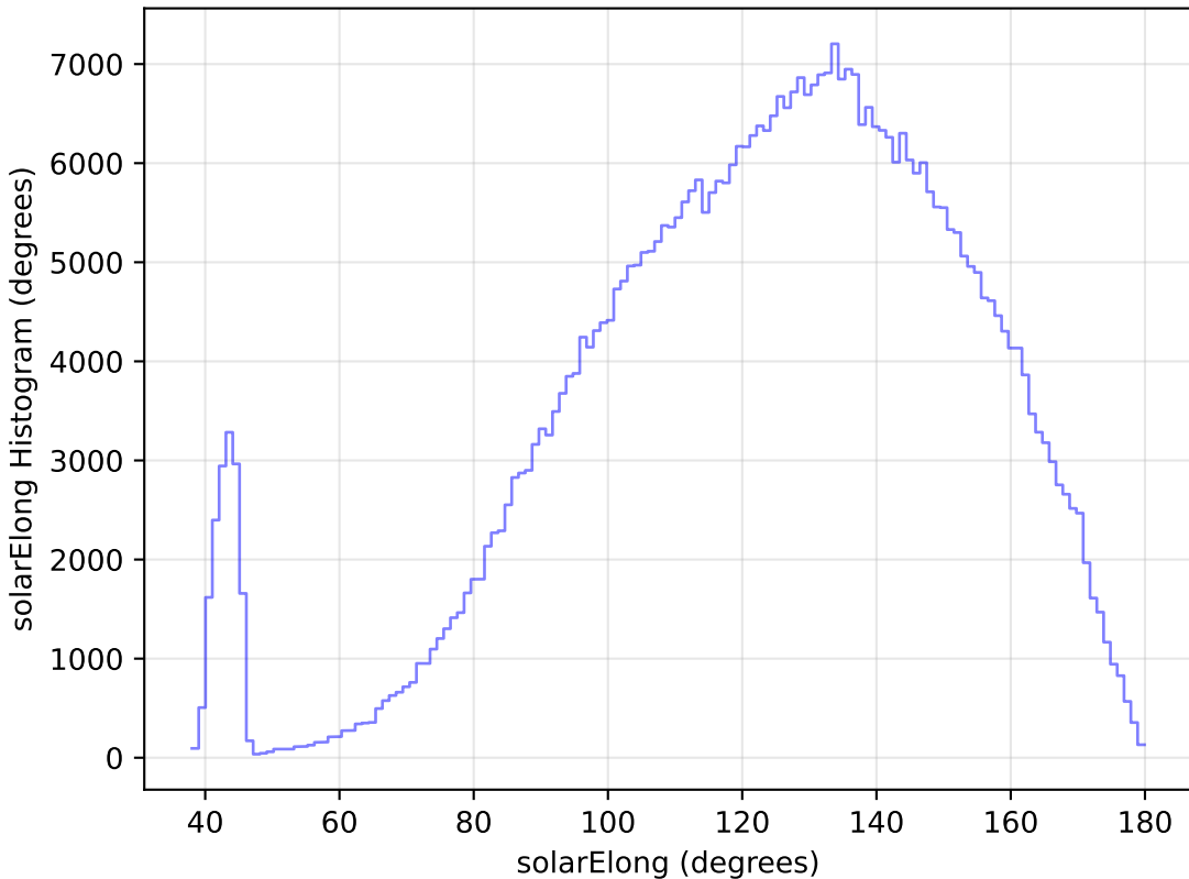
ddf_half_v3.4_10yrs WFD r band: solarElong Histogram
