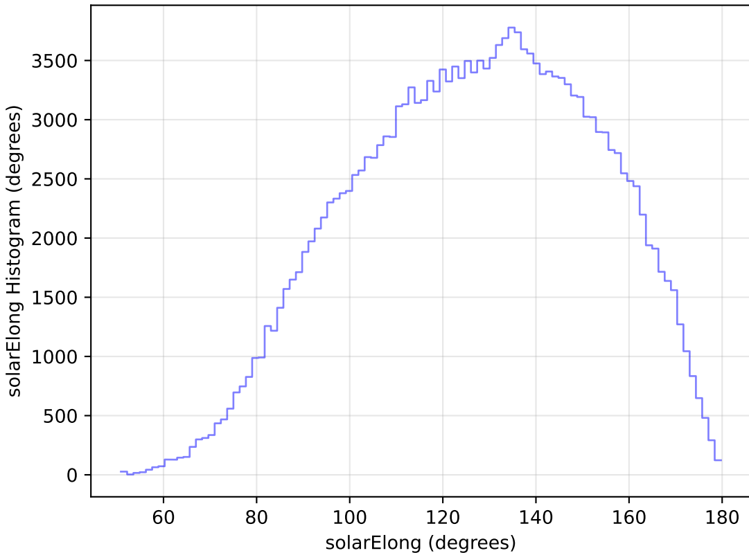
ddf_half_v3.4_10yrs WFD g band: solarElong Histogram
