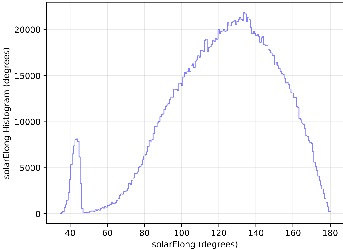
ddf_half_v3.4_10yrs WFD all bands: solarElong Histogram
