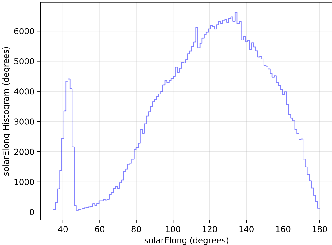
ddf_half_v3.4_10yrs All sky z band: solarElong Histogram
