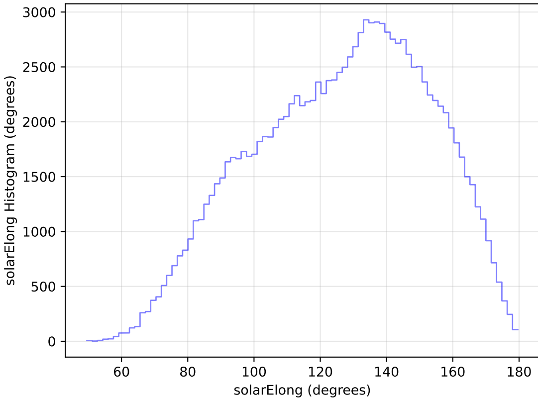
ddf_half_v3.4_10yrs All sky u band: solarElong Histogram
