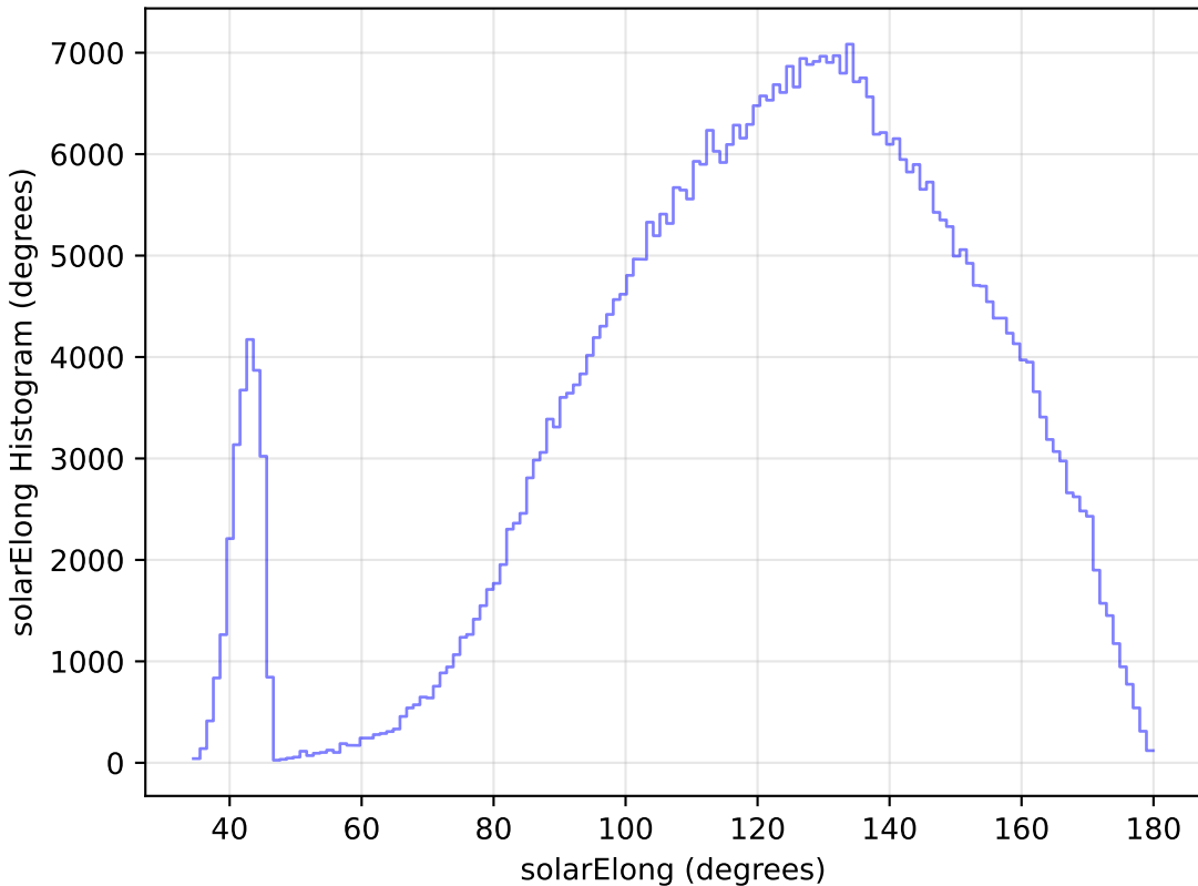
ddf_half_v3.4_10yrs All sky i band: solarElong Histogram
