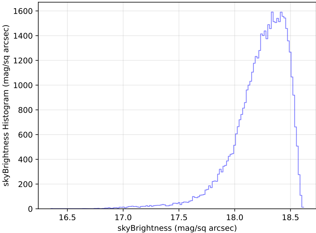
ddf_half_v3.4_10yrs Yr 1 y band: skyBrightness Histogram
