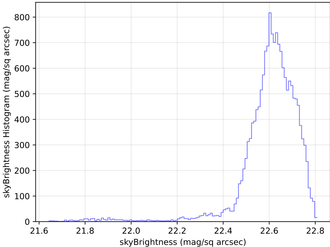
ddf_half_v3.4_10yrs Yr 1 u band: skyBrightness Histogram
