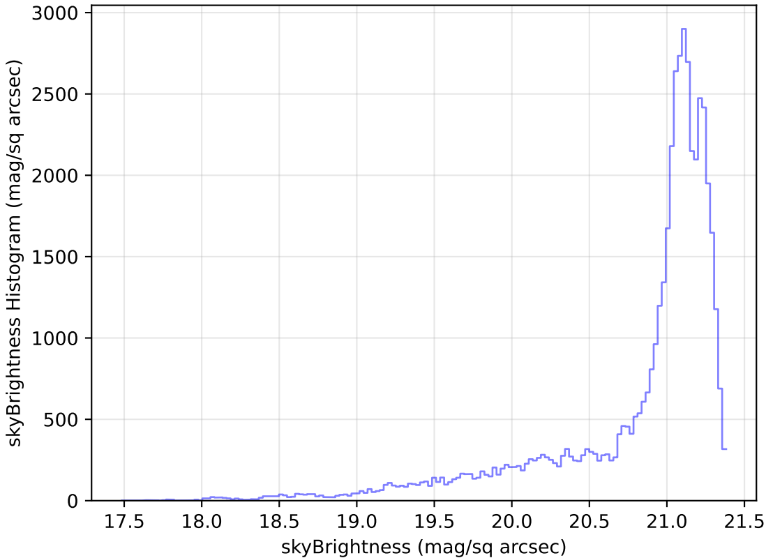
ddf_half_v3.4_10yrs Yr 1 r band: skyBrightness Histogram
