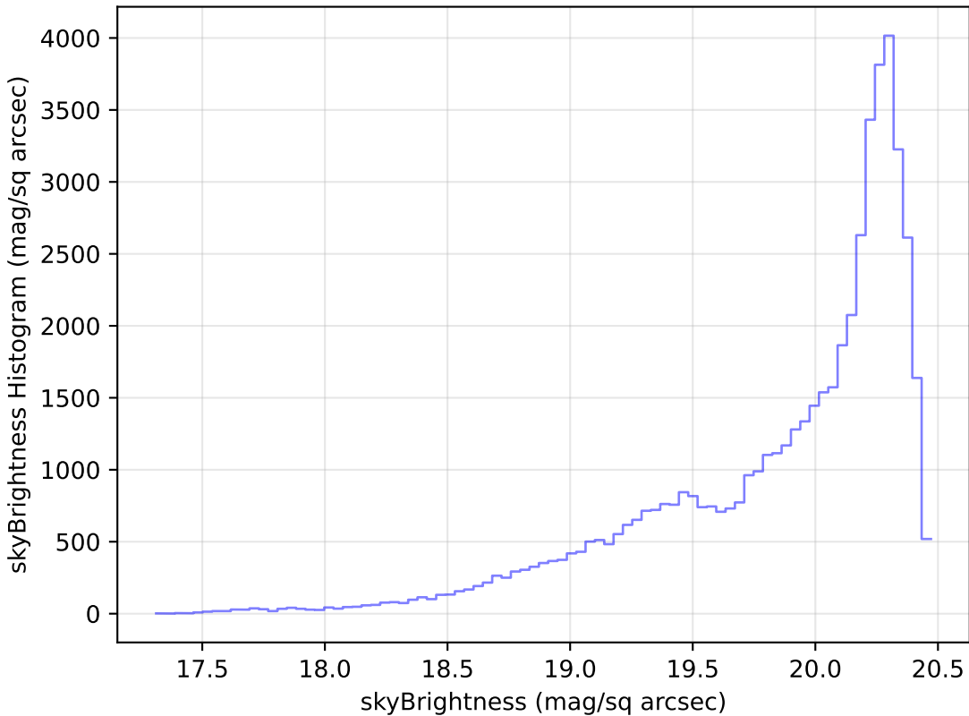
ddf_half_v3.4_10yrs Yr 1 i band: skyBrightness Histogram
