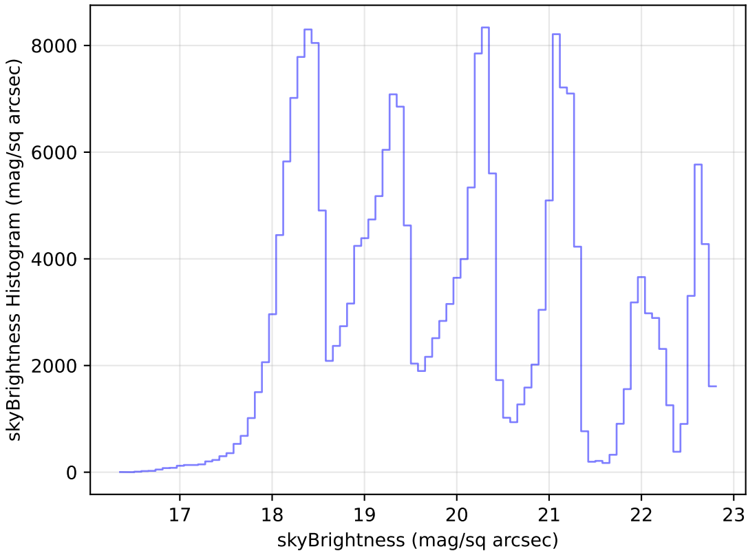
ddf_half_v3.4_10yrs Yr 1 all bands: skyBrightness Histogram
