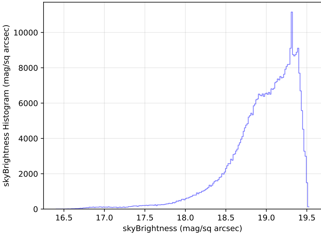
ddf_half_v3.4_10yrs WFD z band: skyBrightness Histogram
