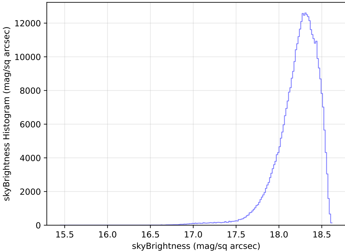
ddf_half_v3.4_10yrs WFD y band: skyBrightness Histogram
