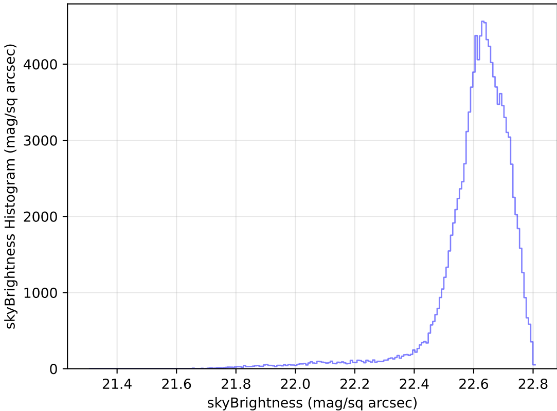
ddf_half_v3.4_10yrs WFD u band: skyBrightness Histogram
