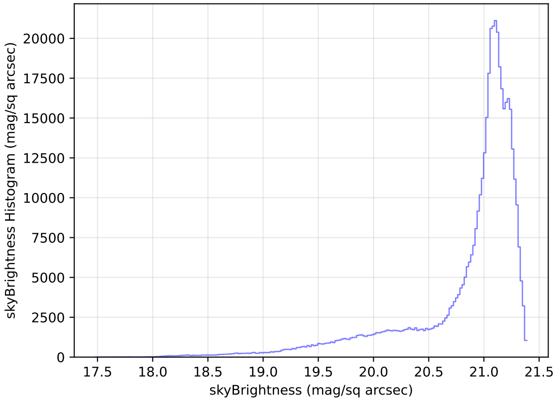
ddf_half_v3.4_10yrs WFD r band: skyBrightness Histogram
