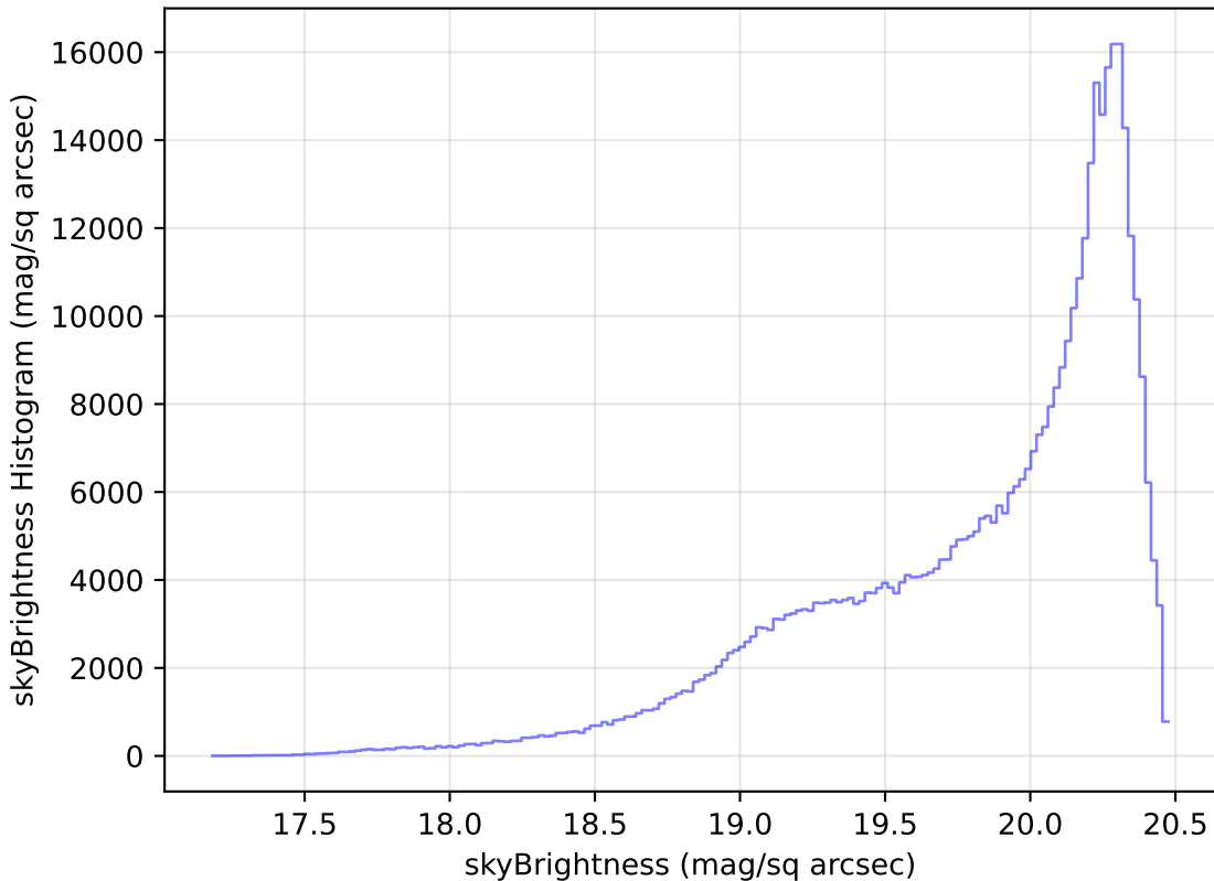
ddf_half_v3.4_10yrs WFD i band: skyBrightness Histogram
