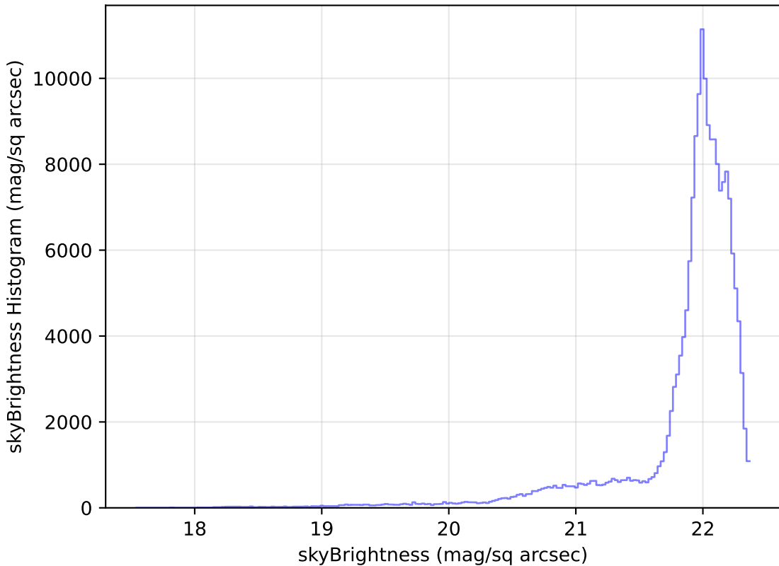
ddf_half_v3.4_10yrs WFD g band: skyBrightness Histogram
