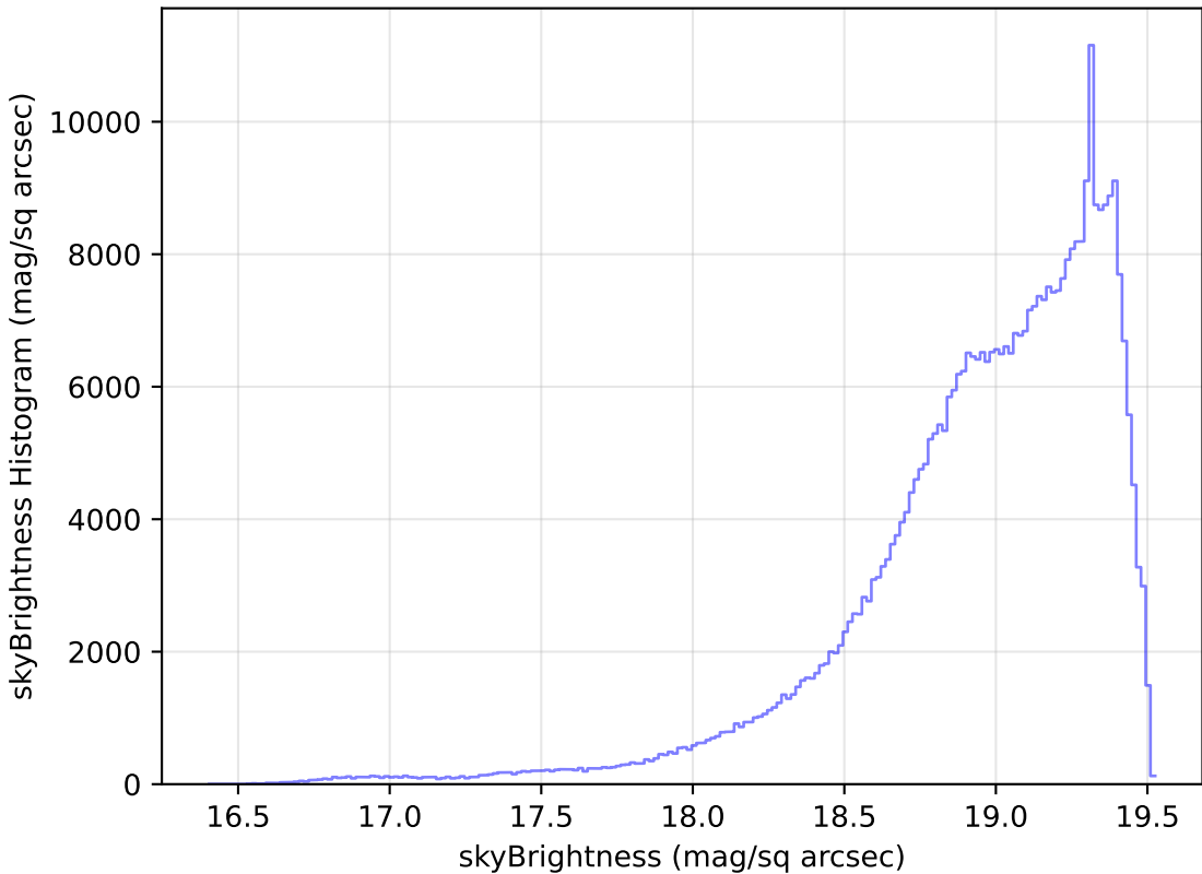
ddf_half_v3.4_10yrs All sky z band: skyBrightness Histogram
