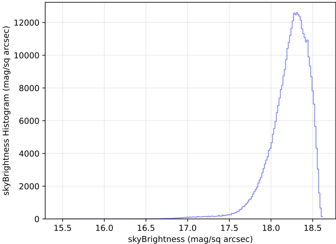
ddf_half_v3.4_10yrs All sky y band: skyBrightness Histogram
