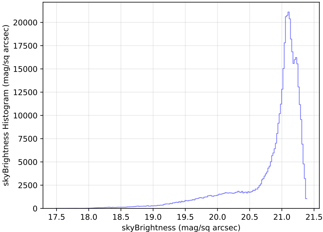
ddf_half_v3.4_10yrs All sky r band: skyBrightness Histogram
